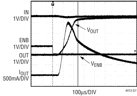
ENB Turn-On, 240µs to Recover with 180mA Load
