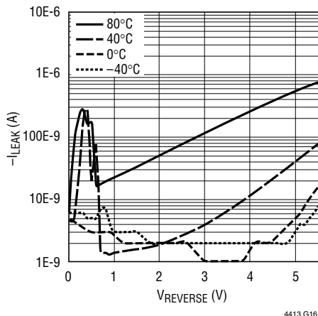
-I LEAK vs V REVERSE
