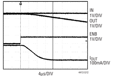
ENB Turn-Off, 16µs to Disconnect IN from 180mA Load
