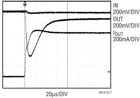
Response to 800mA Load Step in 80µs
