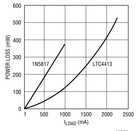
Power Loss LTC4413 vs 1N5817
